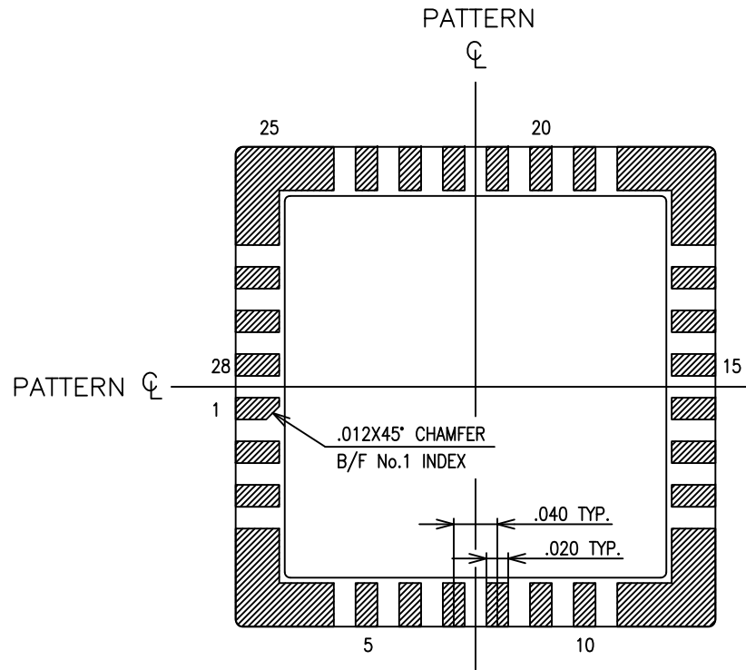
BONDING PATTERN
