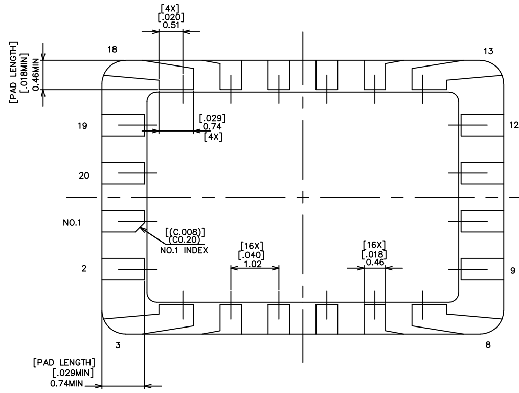
B/G PADS DETAIL
