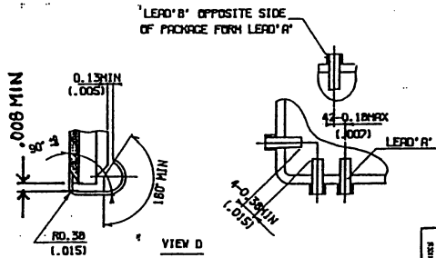
VIEW D
