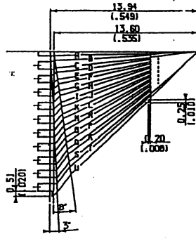
LEAD TIP DETAIL
