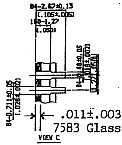
VIEW C
