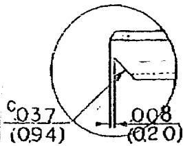
VIEW "R"
