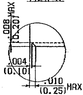
VIEW "P"
