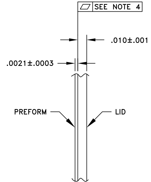
ASSEMBLY ATTACH ITEM 2 TO ITEM 1 SCALE 4:1
