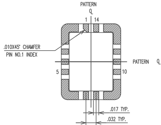
BONDING PATTERN
